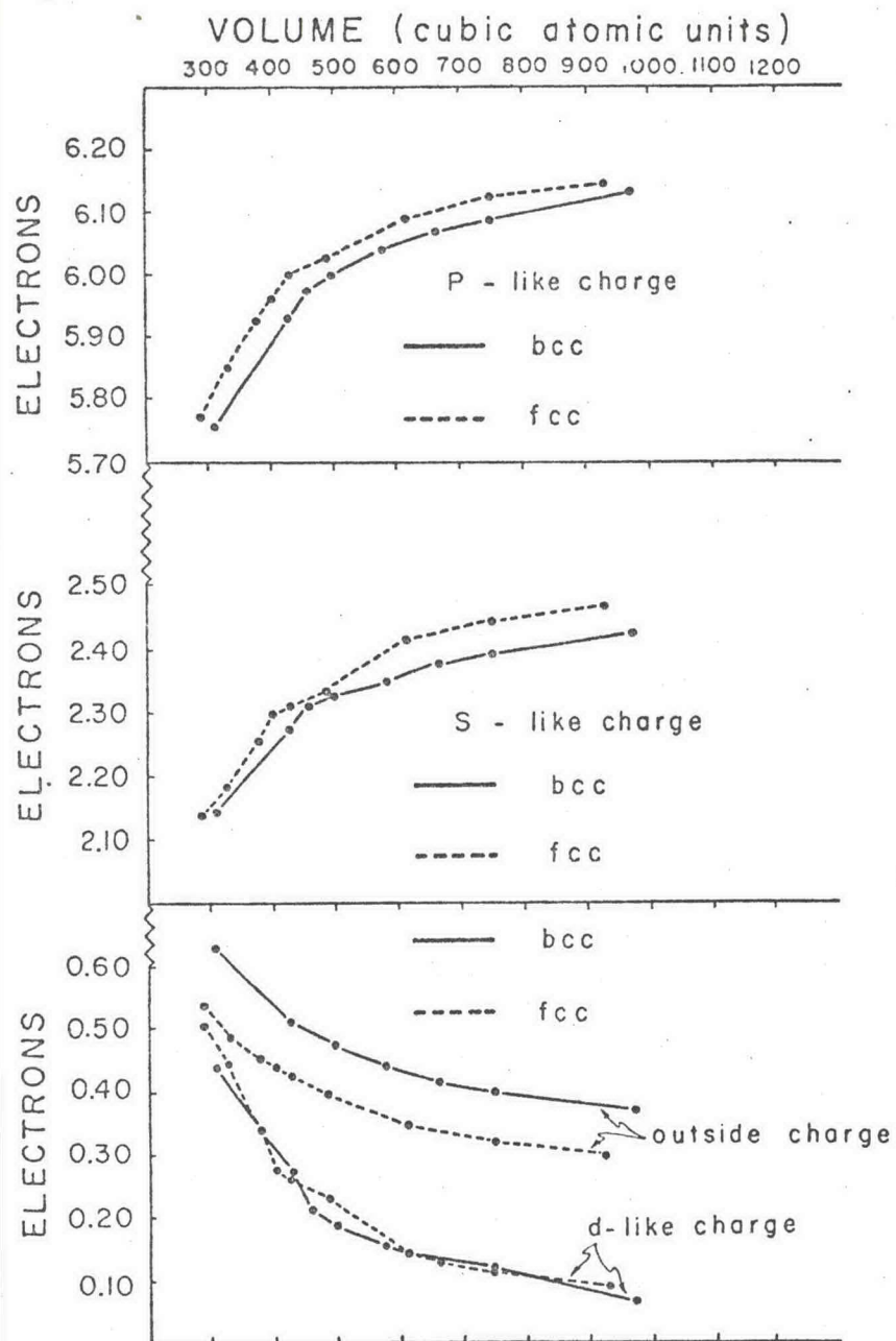
FIG. 3. Cs charge components.
