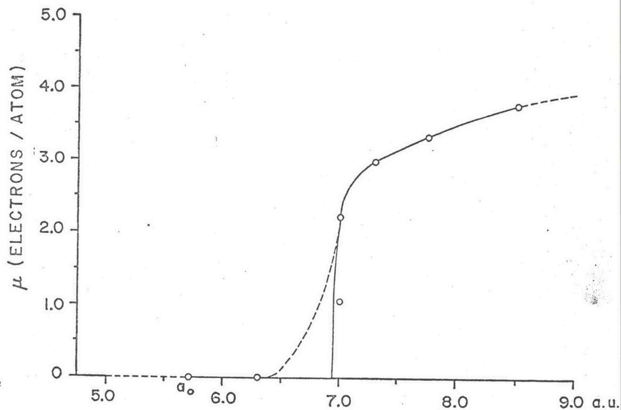
FIG. 4. V magnetic moment.
